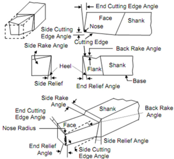
Figure 1: Geometry of single point cutting tool Source:www.expertsmind.com
